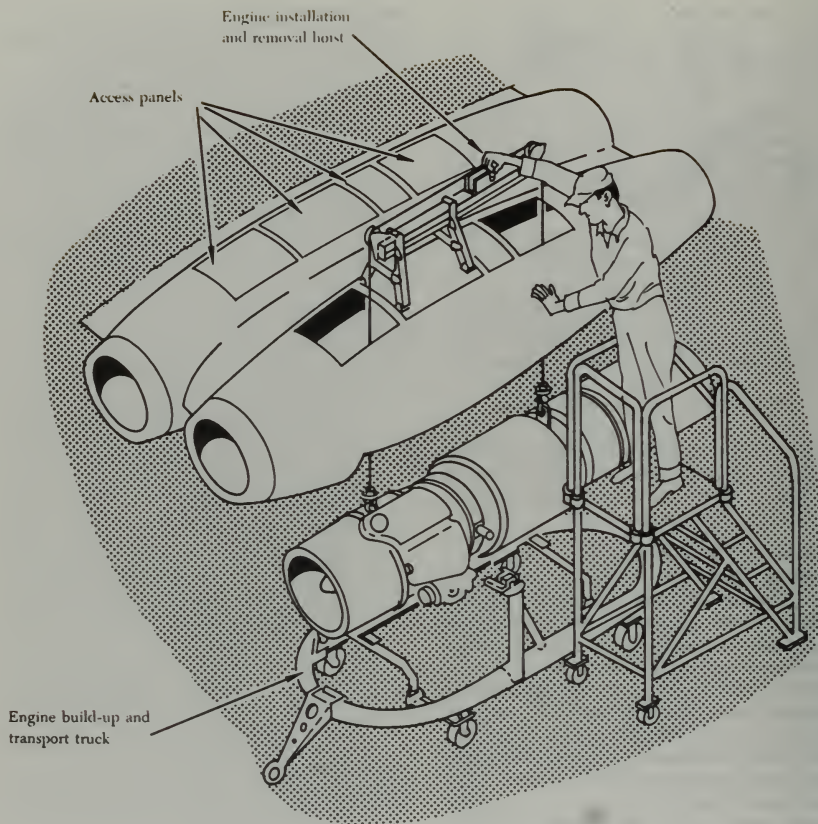
FIGURE 8-19. Installation with a two-cable hoist.
